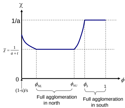
Figure 4: Global Emissions (Tax)
