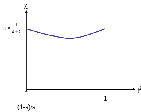
Figure 12: Emissions and Voluntary Tax
