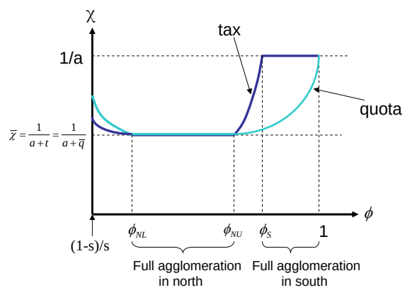
Figure 10: Global Emissions with Tax and Quota
