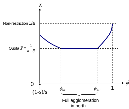
Figure 8: Global Emissions (quota)
